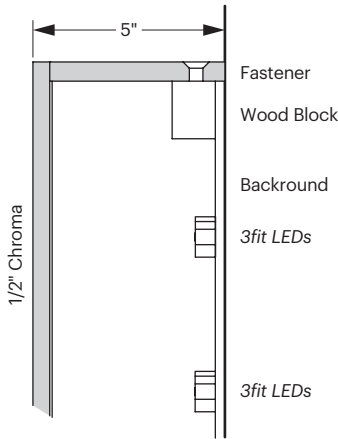
Section View *Spacing of the lights is specific to the translucency of the resin. Contact 3form for more information.
