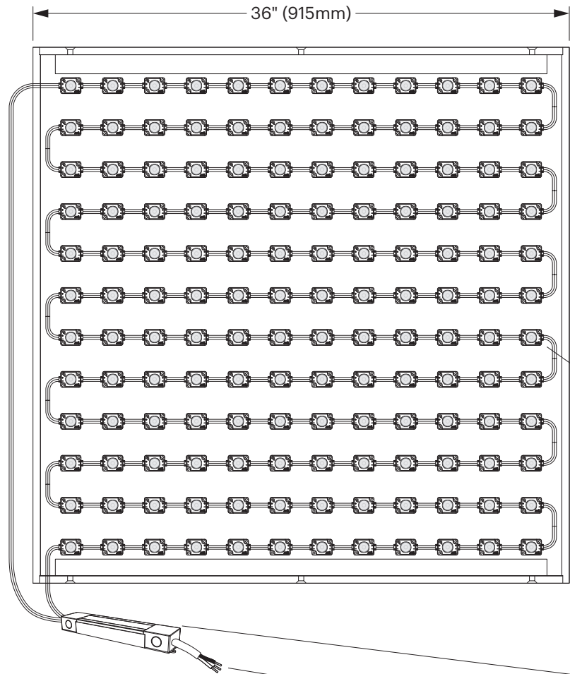
White LED 3fit Overall View
